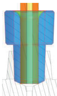
Tube Tuck Connector with 1/16" tubing
